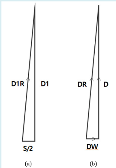
Figure 3: (a) D1R is the one-way distance travelled by light source A from mirror b to mirror a without any external influence. (b) D is the total distance travelled by light source A without any external influence. DW is the total distance travelled by the wind. DR is the total distance travelled by light source A actually due to the external influence (wind). Here, the travel times ( t ) of D, DW, and DR are the same.
